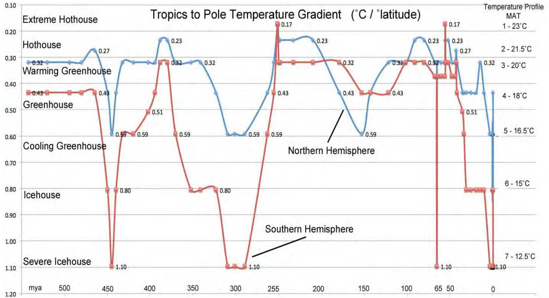
Figure 14. Tropics to Pole Temperature Gradient ( ^{\circ}\text{C}/^{\circ}\text{latitude} ) estimated from paleoclimatic reconstructions (Boucot et al., 2013). Southern Hemisphere (red), Northern Hemisphere (blue). The corresponding Temperature Profile and associated Mean Annual Temperature are plotted along the right side of the chart.
